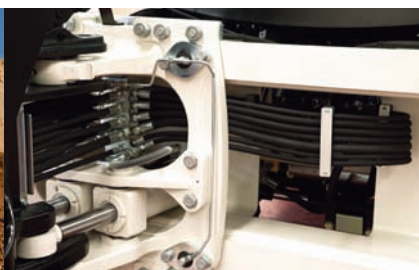
Heavy duty monoblock kingpost carriage with centrally mounted hydraulic cylinders
